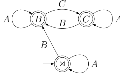
Figure 4.5: Tier based automaton.
