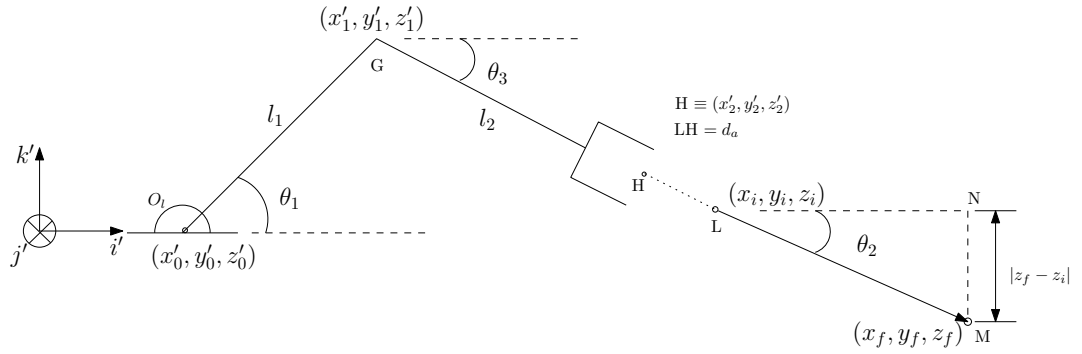
Figure 5.3: Figure showing alignment of Corobot's gripper with the approach vector p_o .
