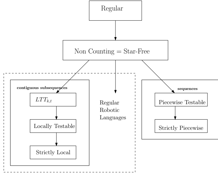
Figure 4.1: Location of regular robotic languages within the Sub-regular hierarchy.
