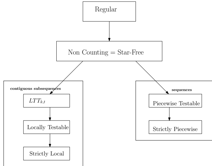
Figure 1.4: The Sub-regular hierarchy of language patterns.
