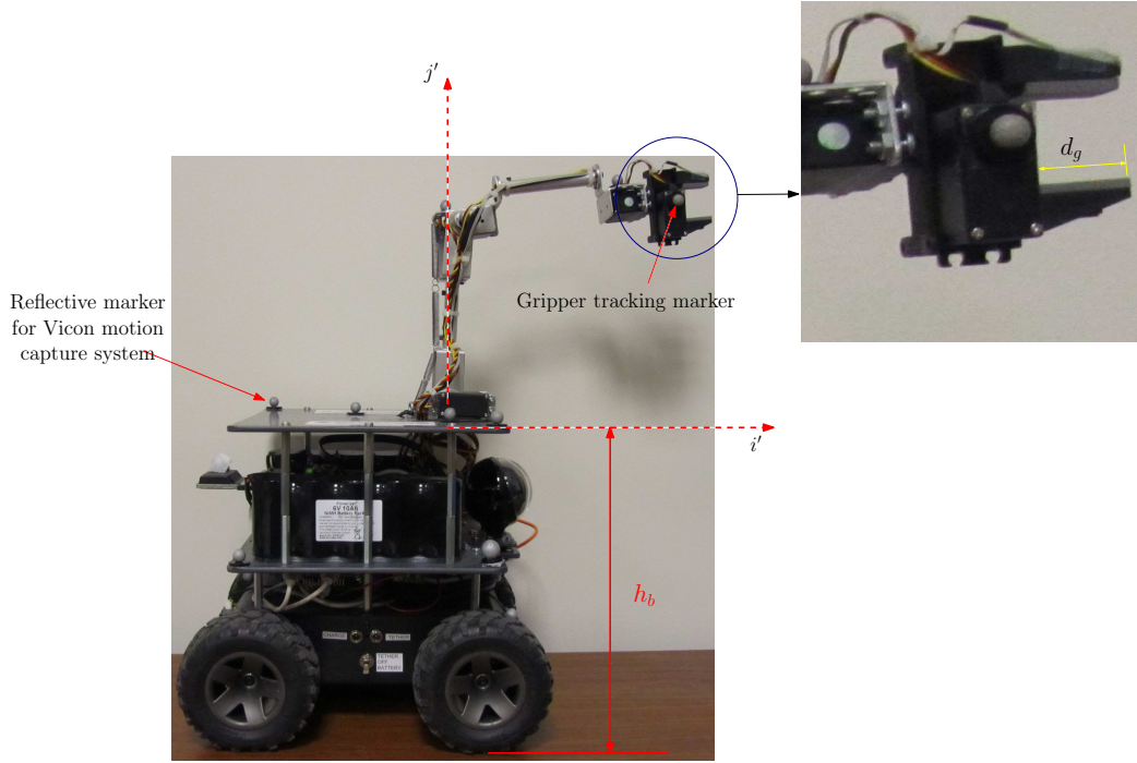
Figure 5.2: The Coroware Corobot used in our case study
