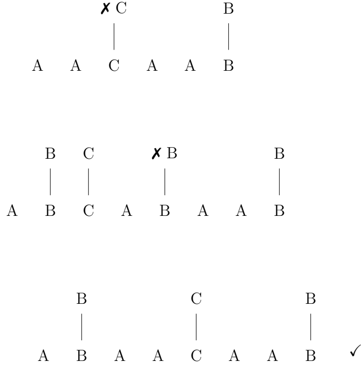
Figure 4.3: Figure describing how autosegments enable a clear understanding of acceptable words.
