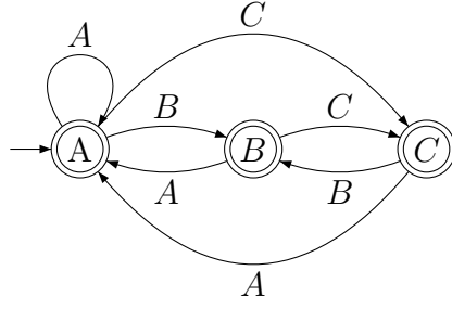
Figure 4.4: SL_2 base tier automaton for the grammar (4.5)
