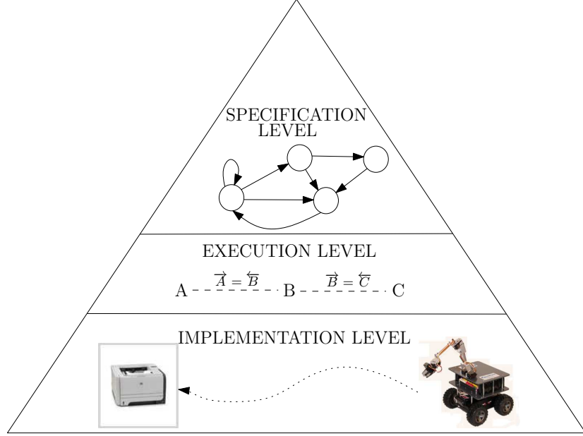
Figure 2.1: Figure showing the hierarchical structure in symbolic control designs, as it would apply to a “fetch-a-printout” example of section 1.1. The specification level describes the overall abstract behavior of the system; the execution level describes feasible sequences of symbols (plans) depending on whether the post-conditions ( \vec{\cdot} ) of one symbol satisfy the pre-conditions ( \overleftarrow{\cdot} ) required by the following symbol; the implementation level executes the plan on an actual system.
